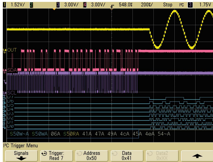
The MSO option lets you see the complex interactions among your signals on up to 20 channels at the same time.
